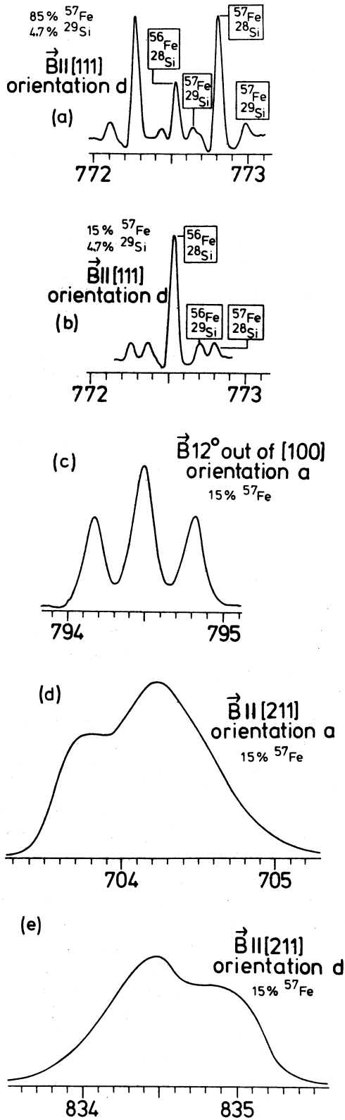
FIG. 2. Line shapes of spectrum NL19 for various resonances of transition 2 \leftrightarrow 3 with \nu = 22.8722 GHz and a sample temperature of 1.4 K.
