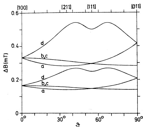
FIG. 5. Calculated angular dependence of the ^{57}\text{Fe} hyperfine lines relative to the central line. The deviations from the measured splittings was less than 0.01 mT.
