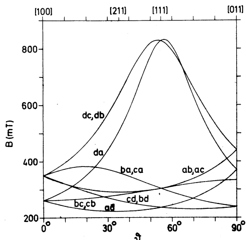
FIG. 6. Calculated angular dependence of spectrum NL21 with \nu = 22.8722 GHz.
